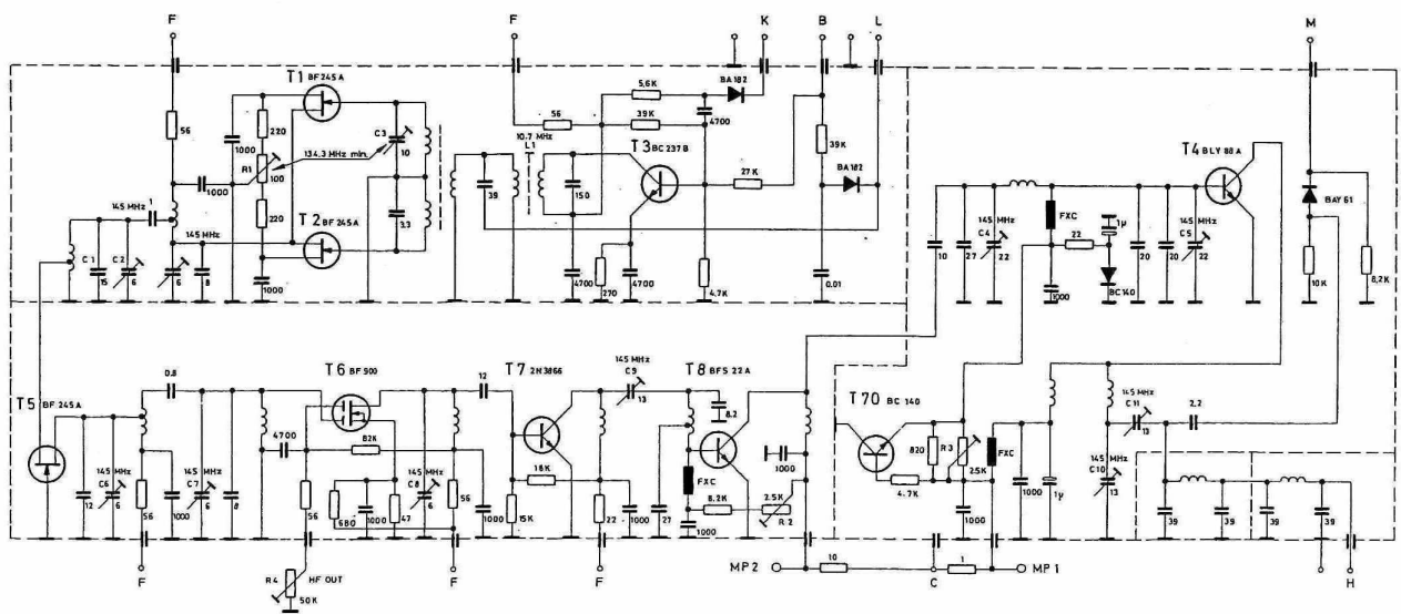
Sender / Transmitter
