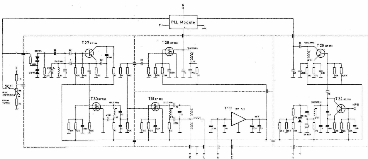
SGO / VCO
